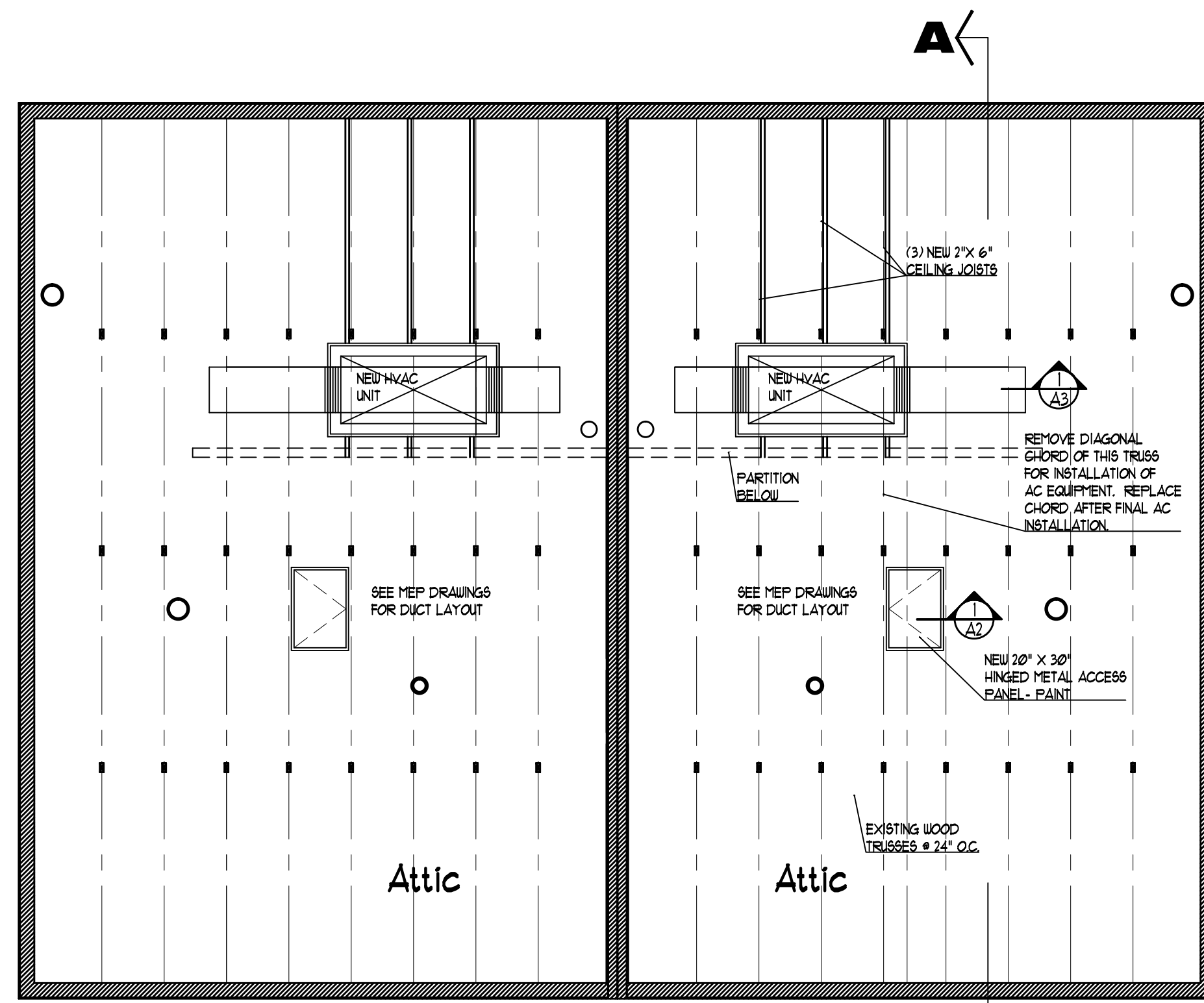
ATTIC PLAN SCALE: 1/4" = 1'-0"
