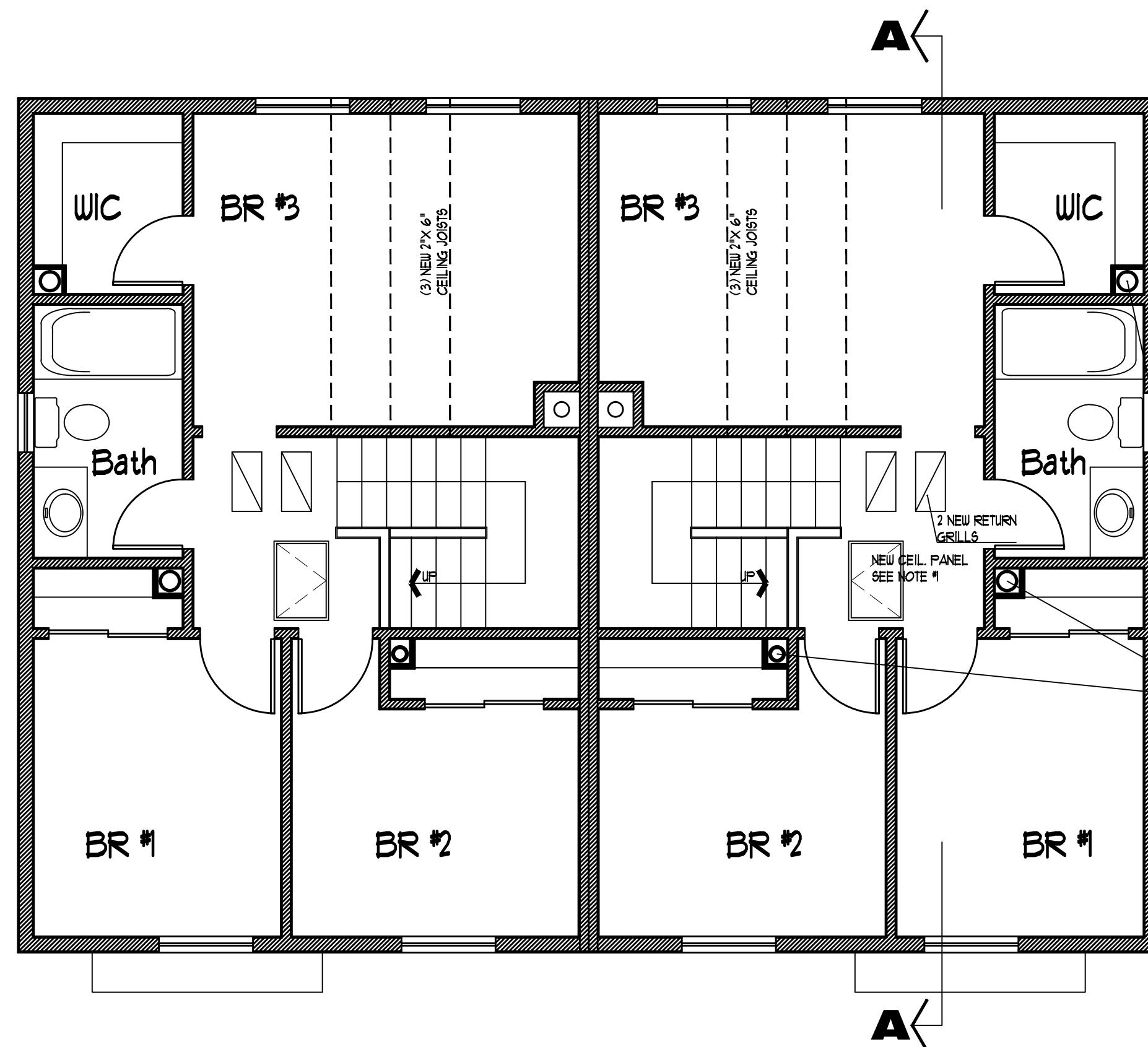
2nd FLOOR PLAN SCALE: 1/4" = 1'-0"
