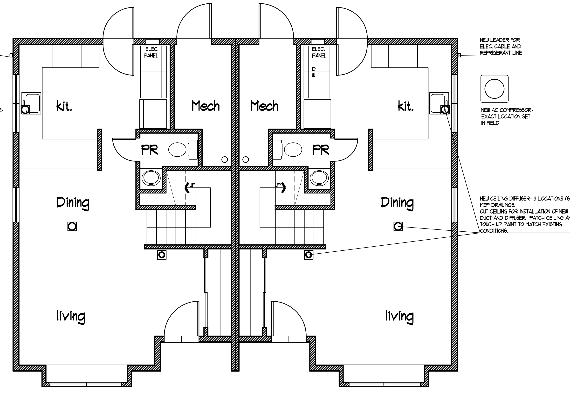
1st FLOOR PLAN SCALE: 1/4" = 1'-0"
