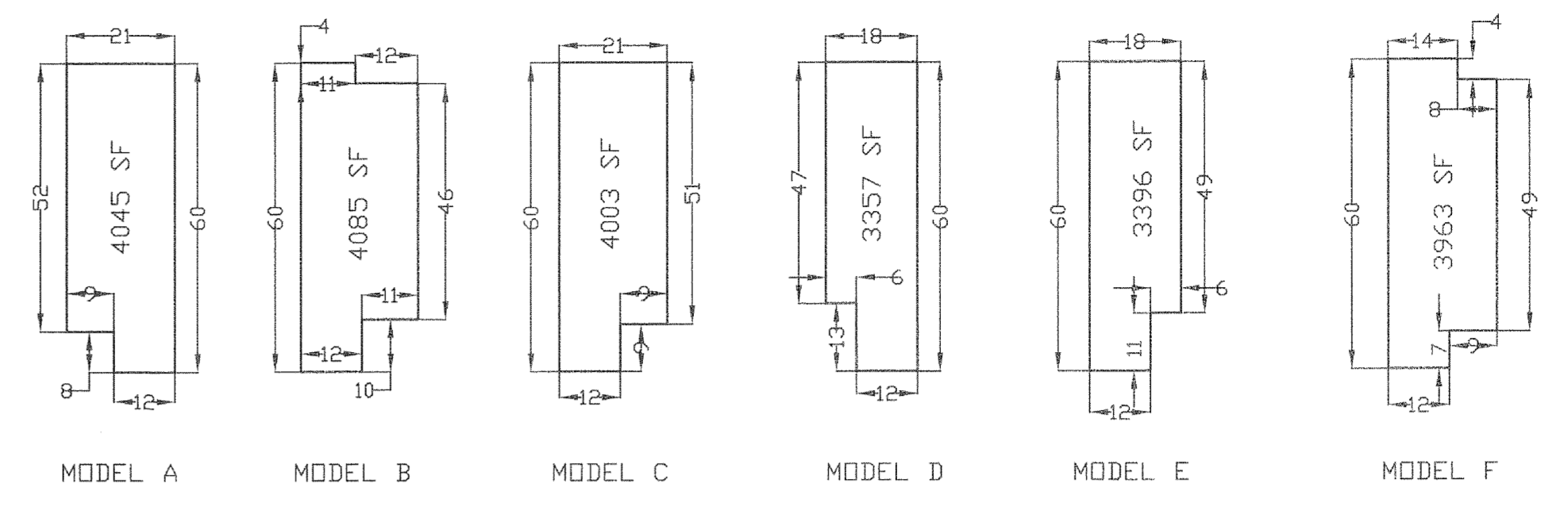
THE MADISON COMMON CONDOMINIUMS UNIT DETAILS 1" = 30'
