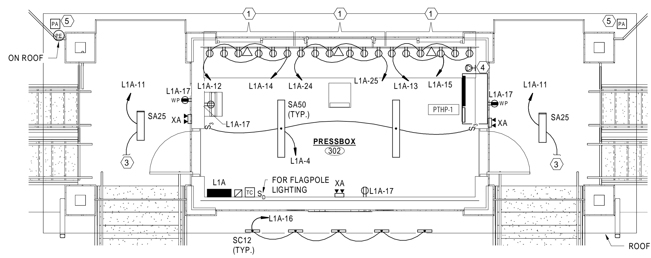
2 BASEBALL - ENLARGED PRESSBOX / SEATING PLAN - ELECTRICAL SCALE: 1/4" = 1'-0"
